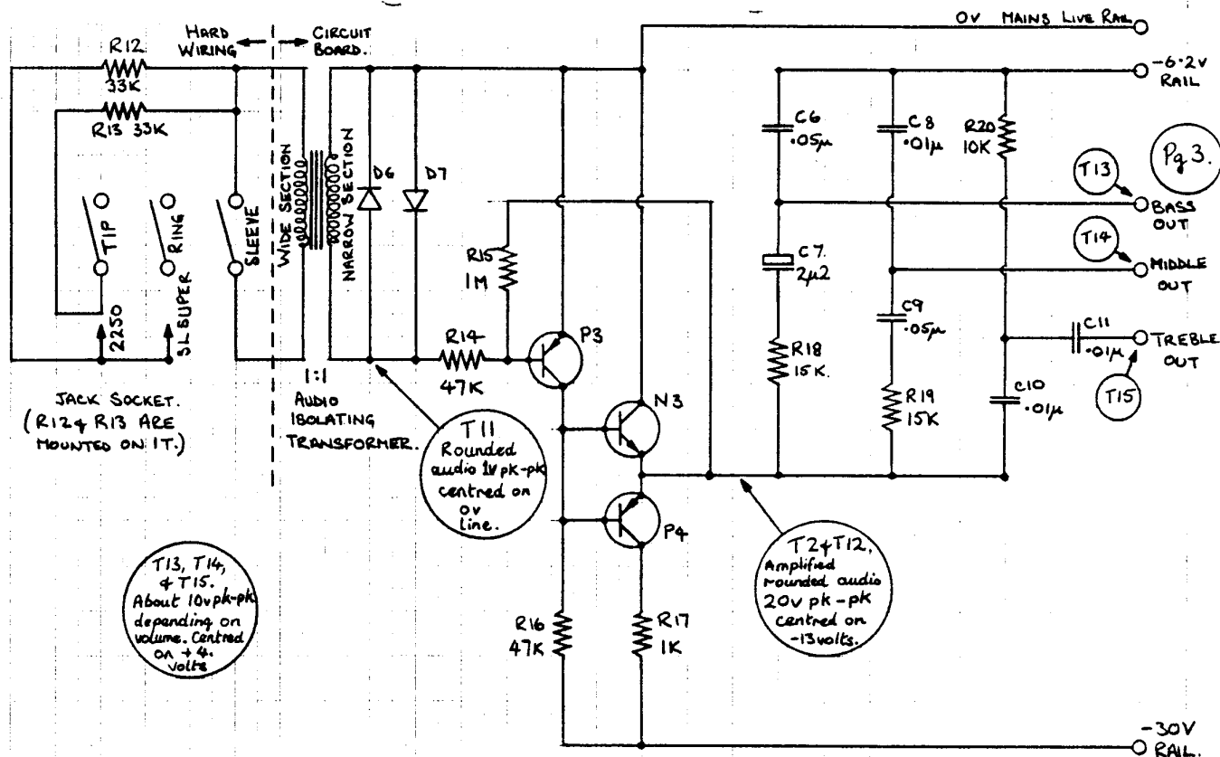
JACK SOCKET & RESISTORS
